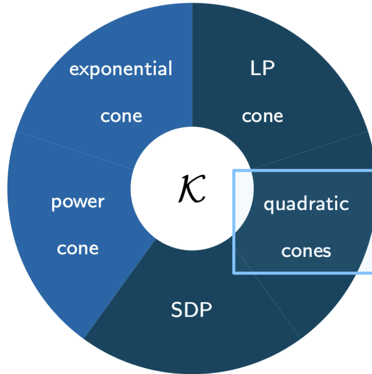
Figure 1. Classification of convex cones. [2]
