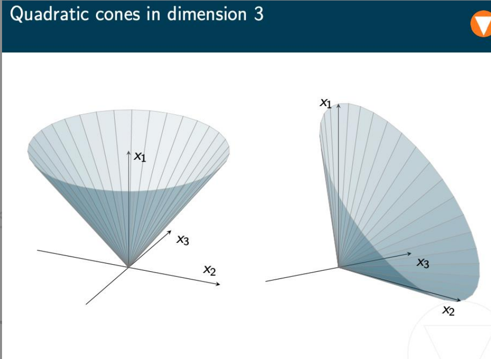
Figure 2. Second order cones in dimension 3. [2]
